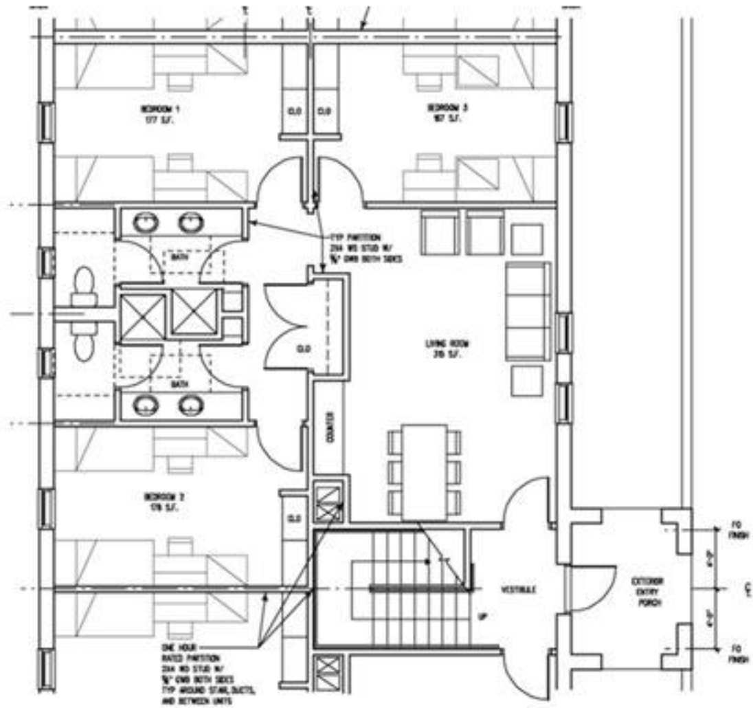
2 A1.2 TYPICAL SUITE UNIT PLAN SCALE 1/4" = 1'-0"
